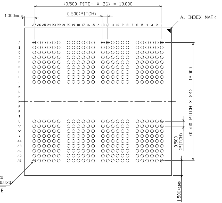
BOTTOM VIEW
