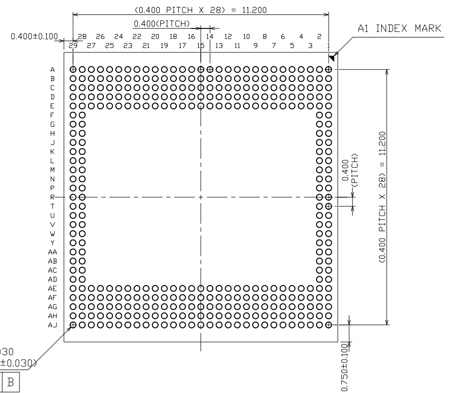
BOTTOM VIEW
